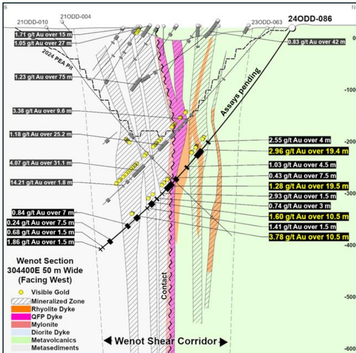
Figure 2. Cross-section for DDH 240DD-086 (partial, additional assays pending)
